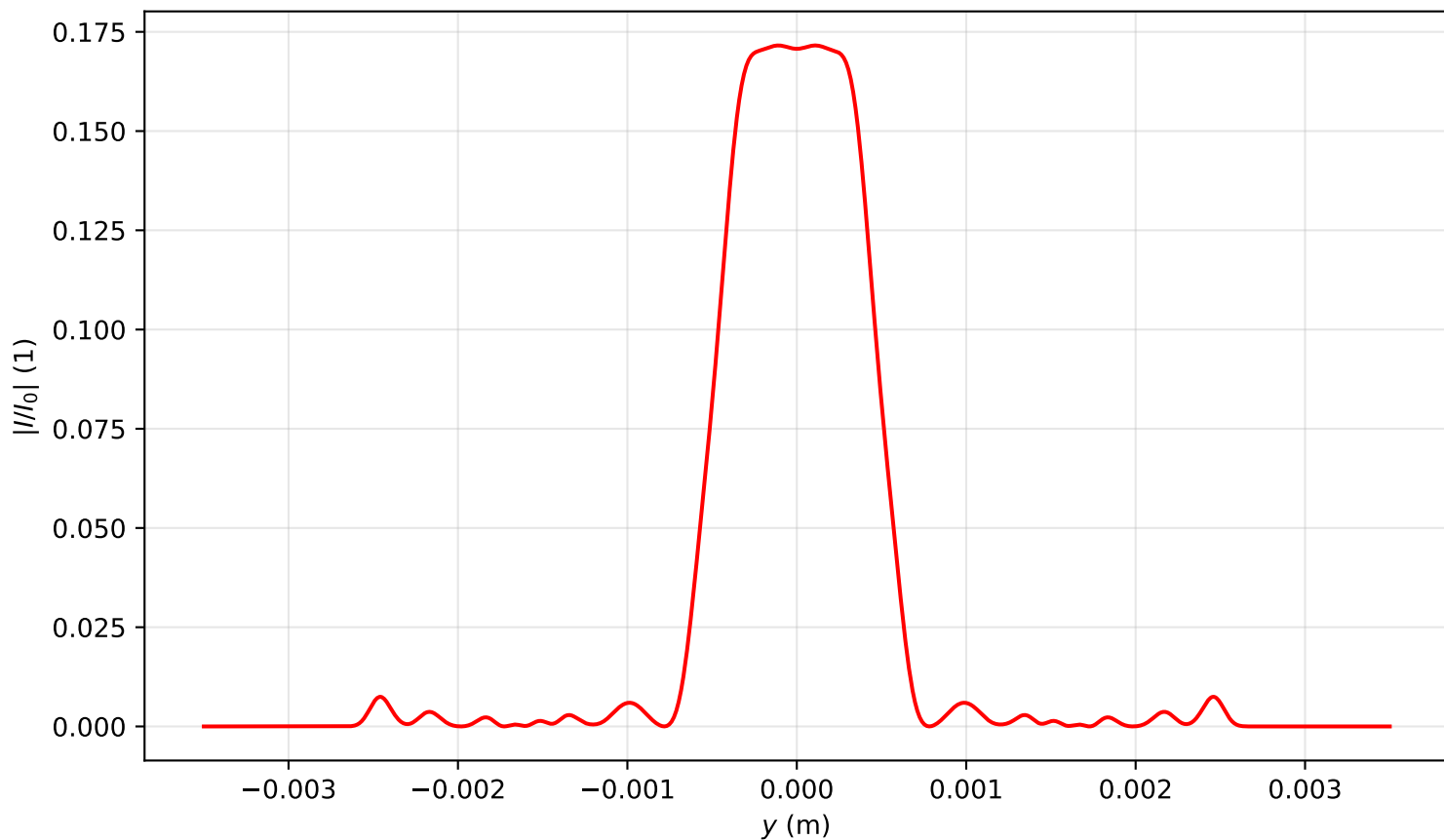
Intensity profile I(x=0, y, z=1.911)/I_0 , P_{in}=5.0P_{cr} , artificial time
